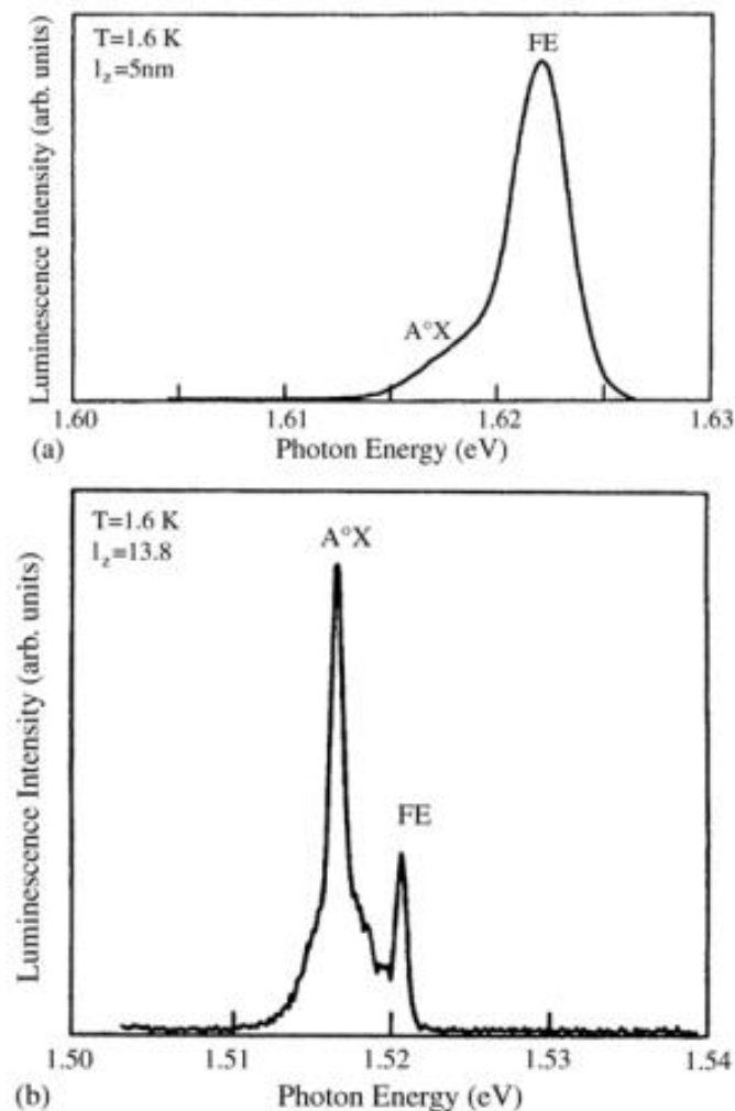
Fig. 14.7. The luminescence of GaAs/Al 1-y Ga y As structures, of two different well width l_z center doped with Be acceptors at low temperature showing the emission from localized intrinsic excitons labelled FE and of acceptor bound excitons (A 0 X) [89H1]
