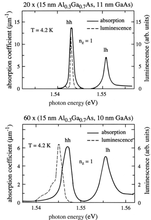
Fig. 15.3. A comparison of absorption and luminescence spectra in two samples of different quality [92O2]
