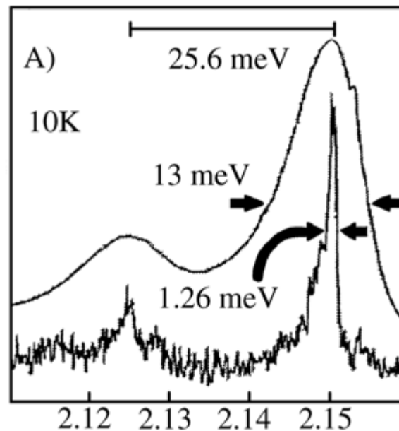
Fig. 15.23. Luminescence spectra of ZnS capped CdSe quantum dots for an ensemble of average radius R = 4.5 nm and of a single dot.
