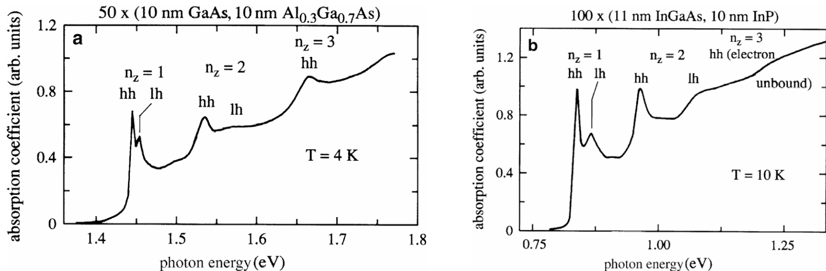
Fig. 15.2 The low temperature absorption spectra of multiple quantum well samples of GaAs/Al 1-y Ga y As (a) and of In 1-y Ga y As/InP (b)
