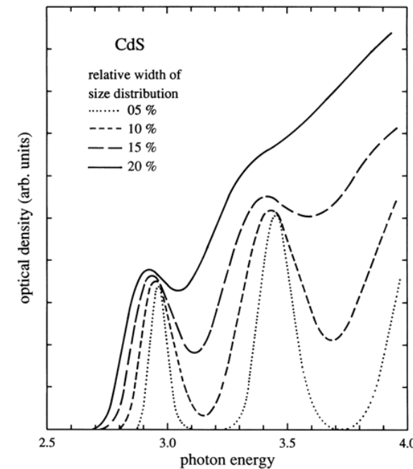
Fig. 15.19. Calculated spectra of the optical density of quantum dots for various relative widths of their size distribution.
